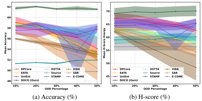
Figure 6. Performance under different OOD ratios.
